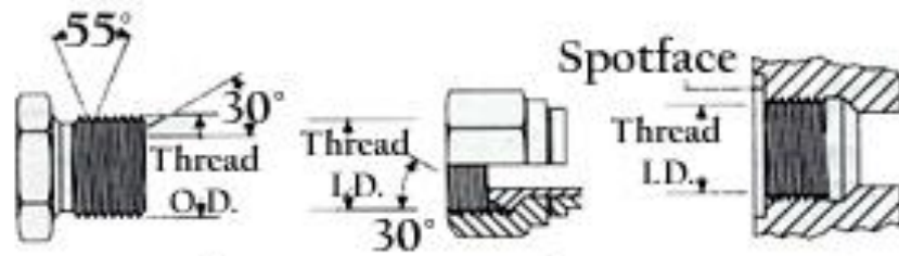
BSPP Male BSPP Female BSPP Female Port
