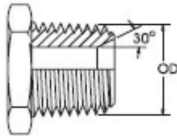
BSPT MALE
